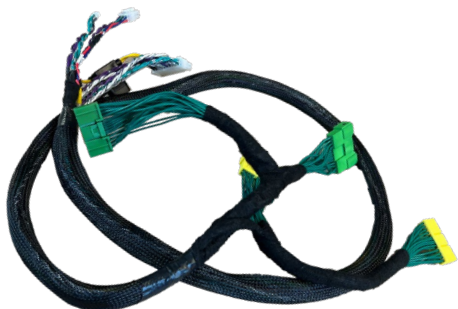
BRS Plug & Play harness
