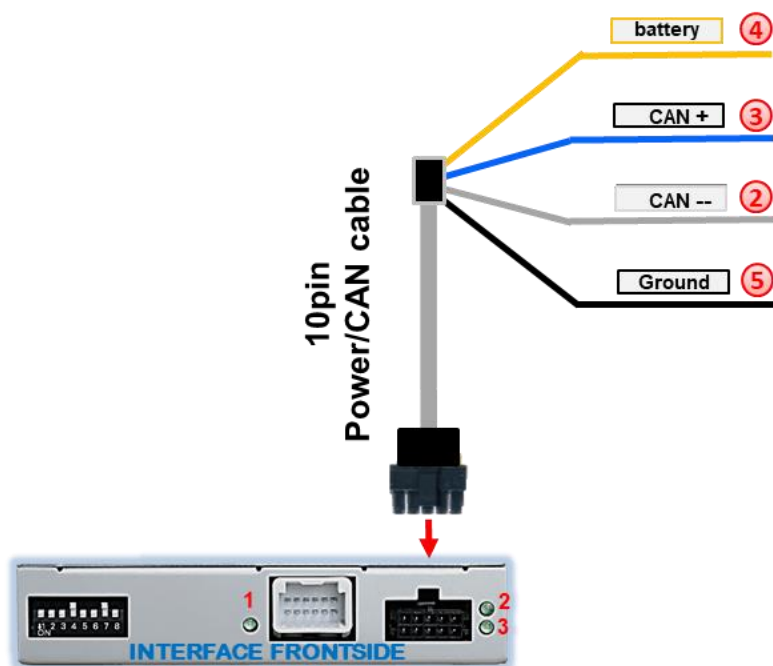
Pin-assignment vehicle harness
