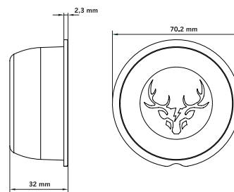
Part No. 830431 SIDE MARKER LED
